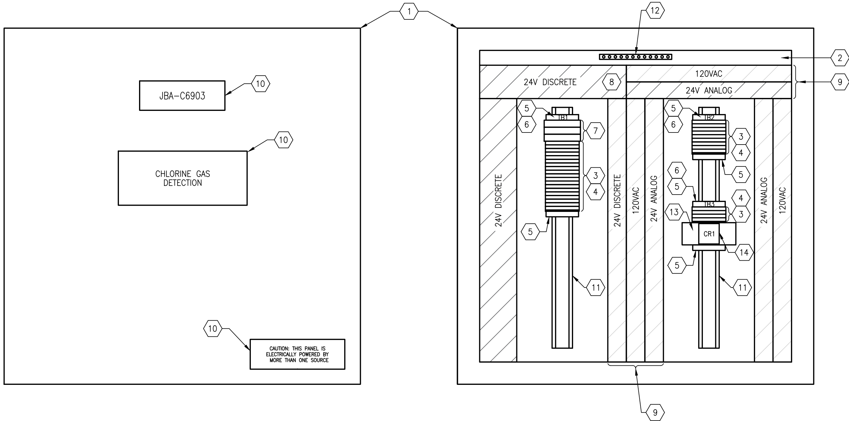
EXTERIOR PANEL VIEW 1 : 4
